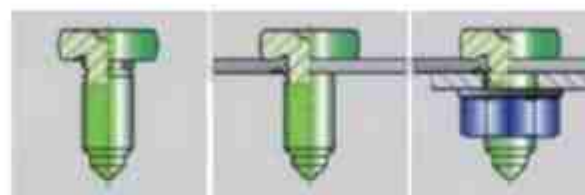
Pressure riveting schematic diagram
