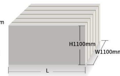
Vertical Tying Bale size (Model XTY-1000W110110-60)
