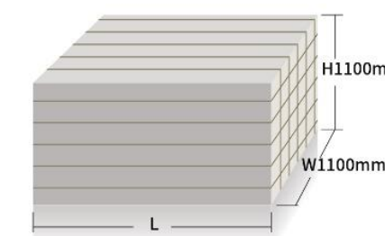
Cross Tying Bale size (Model XTY-1000W110110-60)
